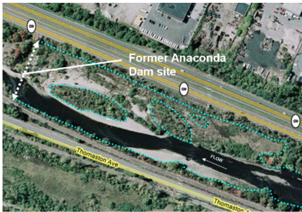
Figure 6. Anaconda Dam site 10 years post removal
