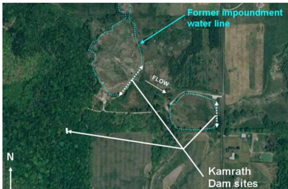
Figure 3. Kamrath Dams site 10 years post removal
